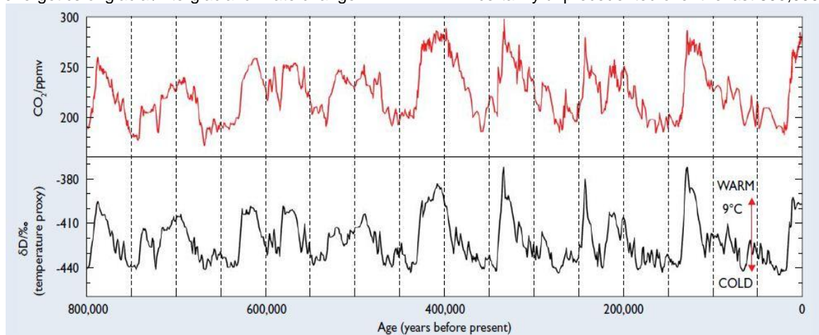
Data Source: Jouzel, J., and others: Orbital and millennial Antarctic climate variability over the last 800,000 years, Science , 317, 793-796, 2007 Lüthi, D., and others: High-resolution carbon dioxide concentration record 650,000-800,000 years before present, Nature , 453, 379-382, 2008
