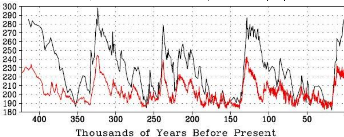
History of Atmospheric CO 2 (Black Line, in Ppmv) and Temperature (Red, in Relative Units) over the Last 420,000 Years from the Vostok Ice Core; After Petit Et Al. (1999)
