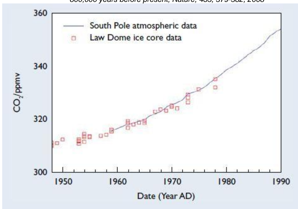
Data Source: MacFarling Meure, C., and others: Law Dome CO 2 , CH 4 and N 2 O ice core records extended to 2,000years BP, Geophys. Res. Lett. , 33, L14810, doi:10.1029/2006GL026152, 2006 Atmospheric data supplied by NOAA/ESRL
